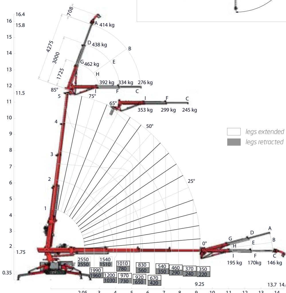
Without counterweight
