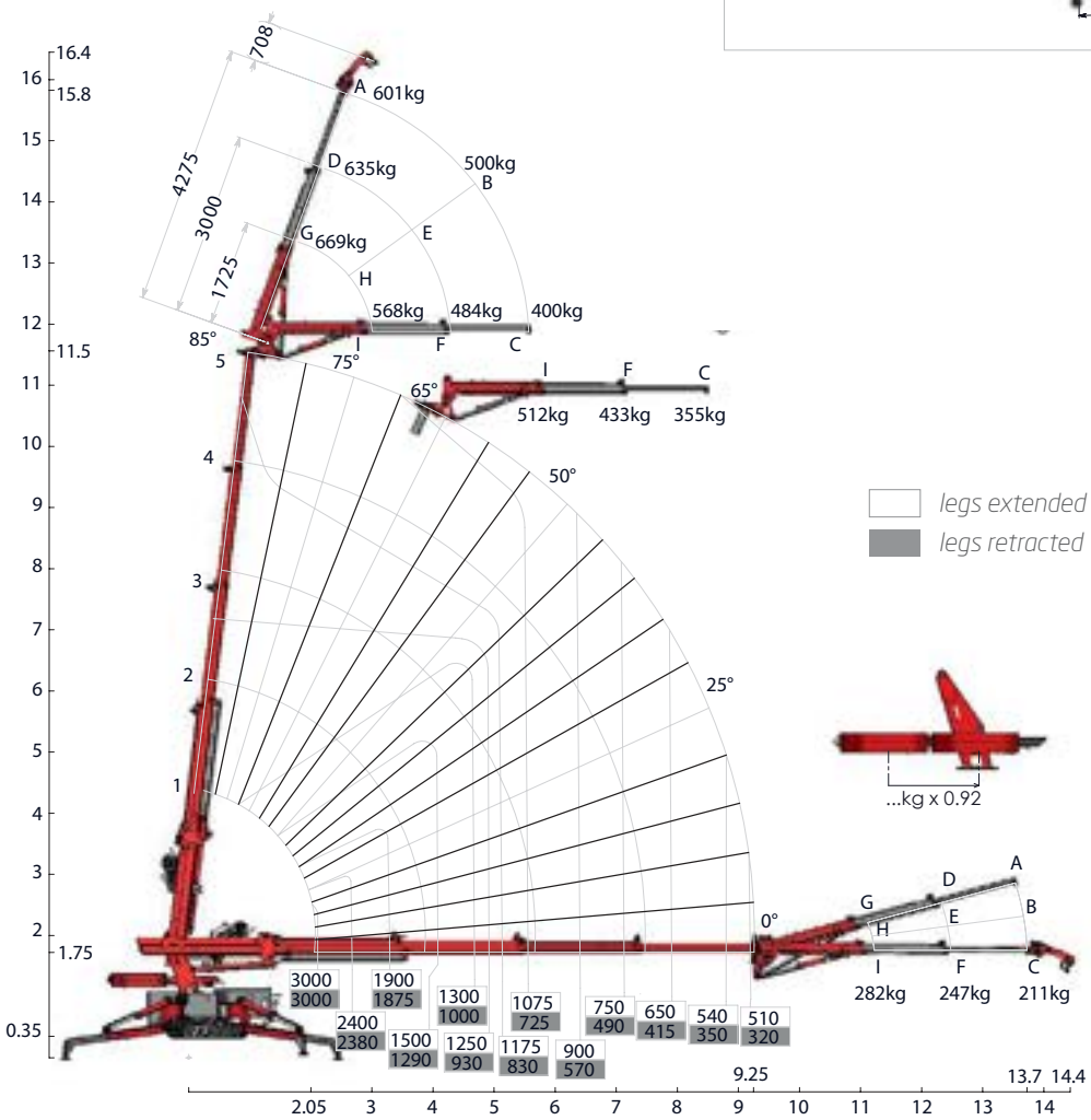
With counterweight
